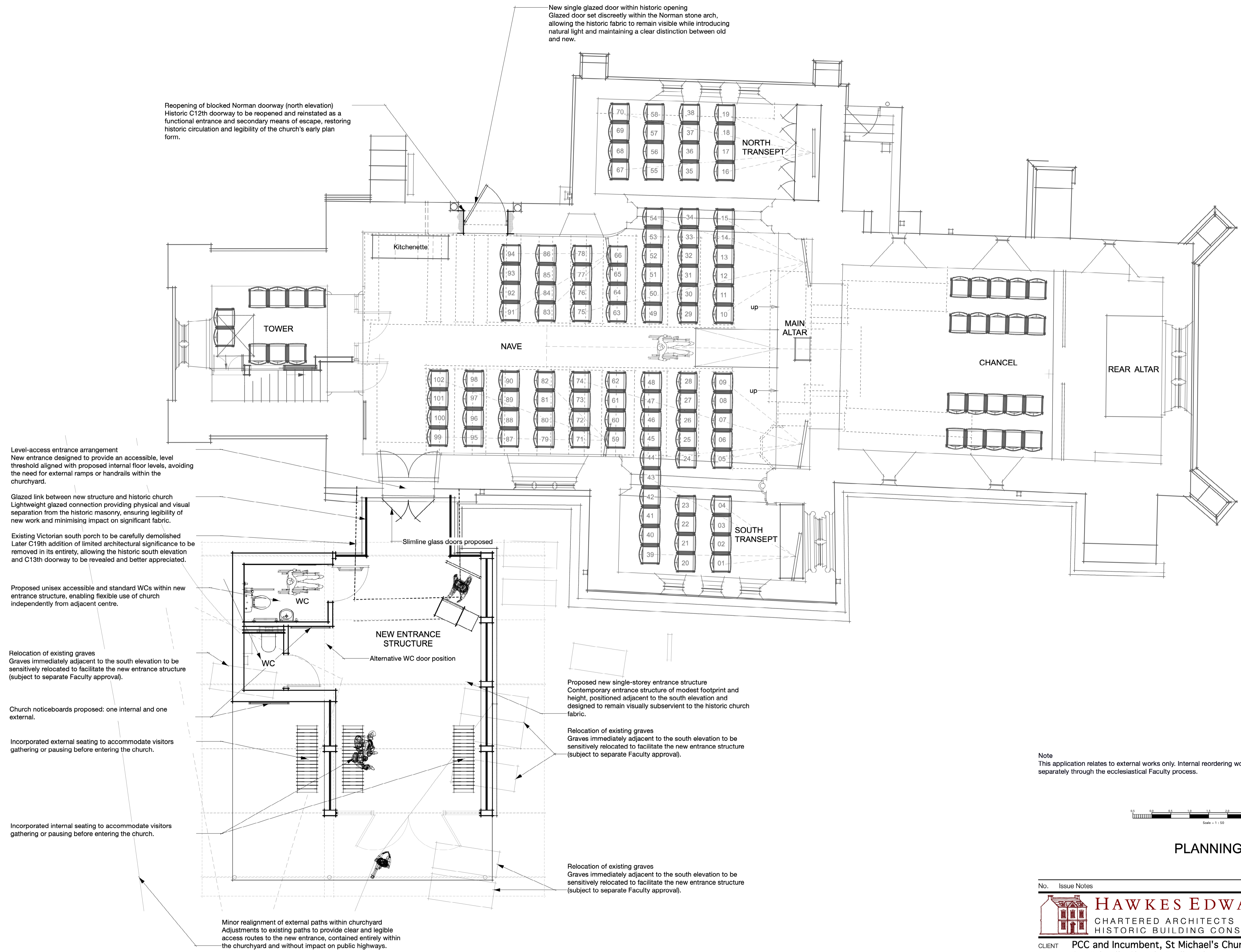
Ground Floor Plan - as Proposed
